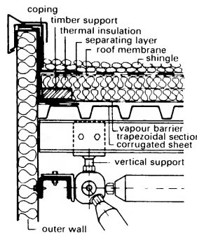
⑥ Structural connections to wall and roof
